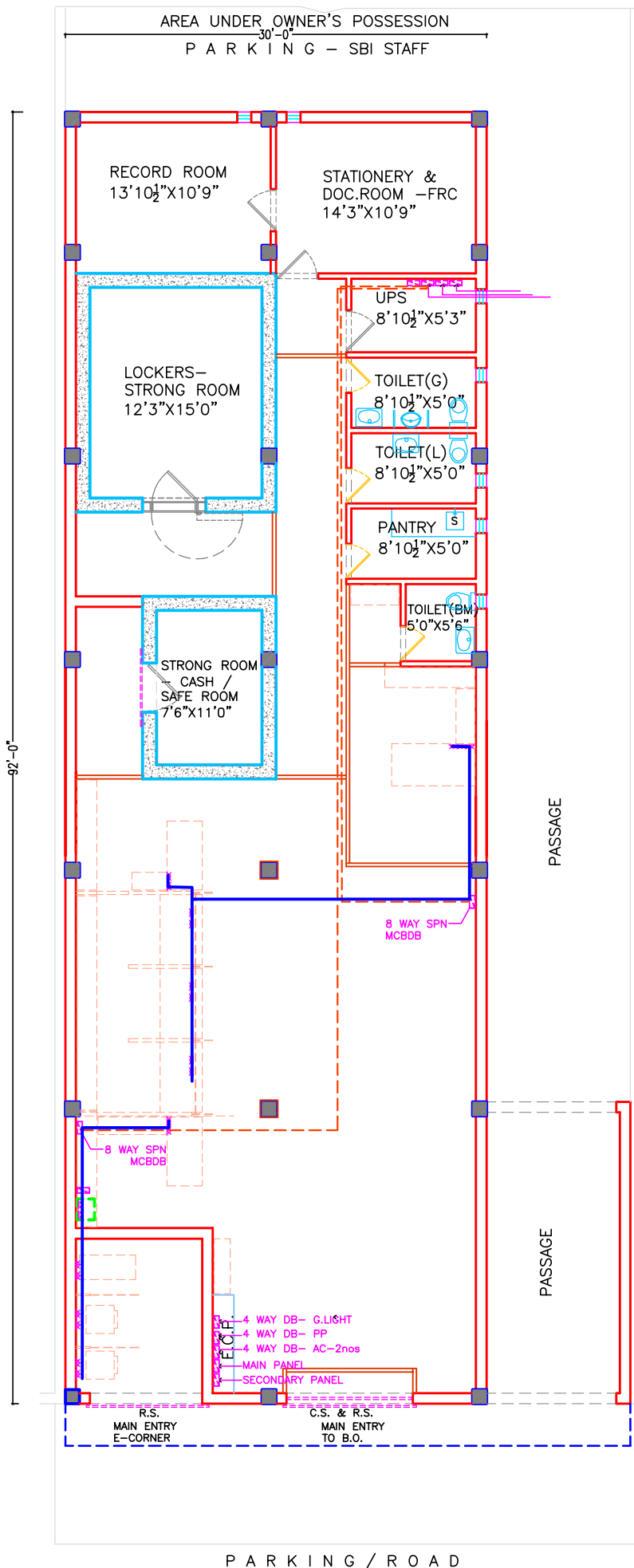
LAYOUT PLAN - G.F.
