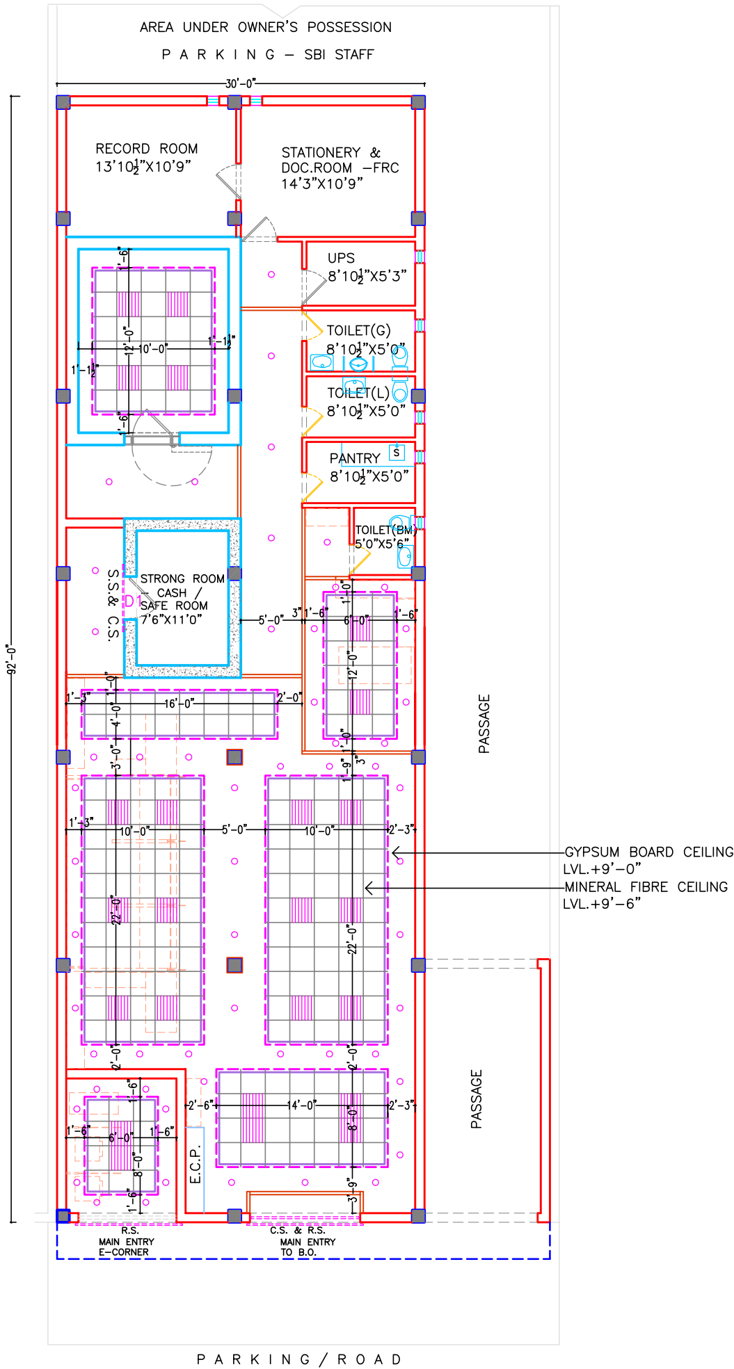
LAYOUT PLAN - G.F.
