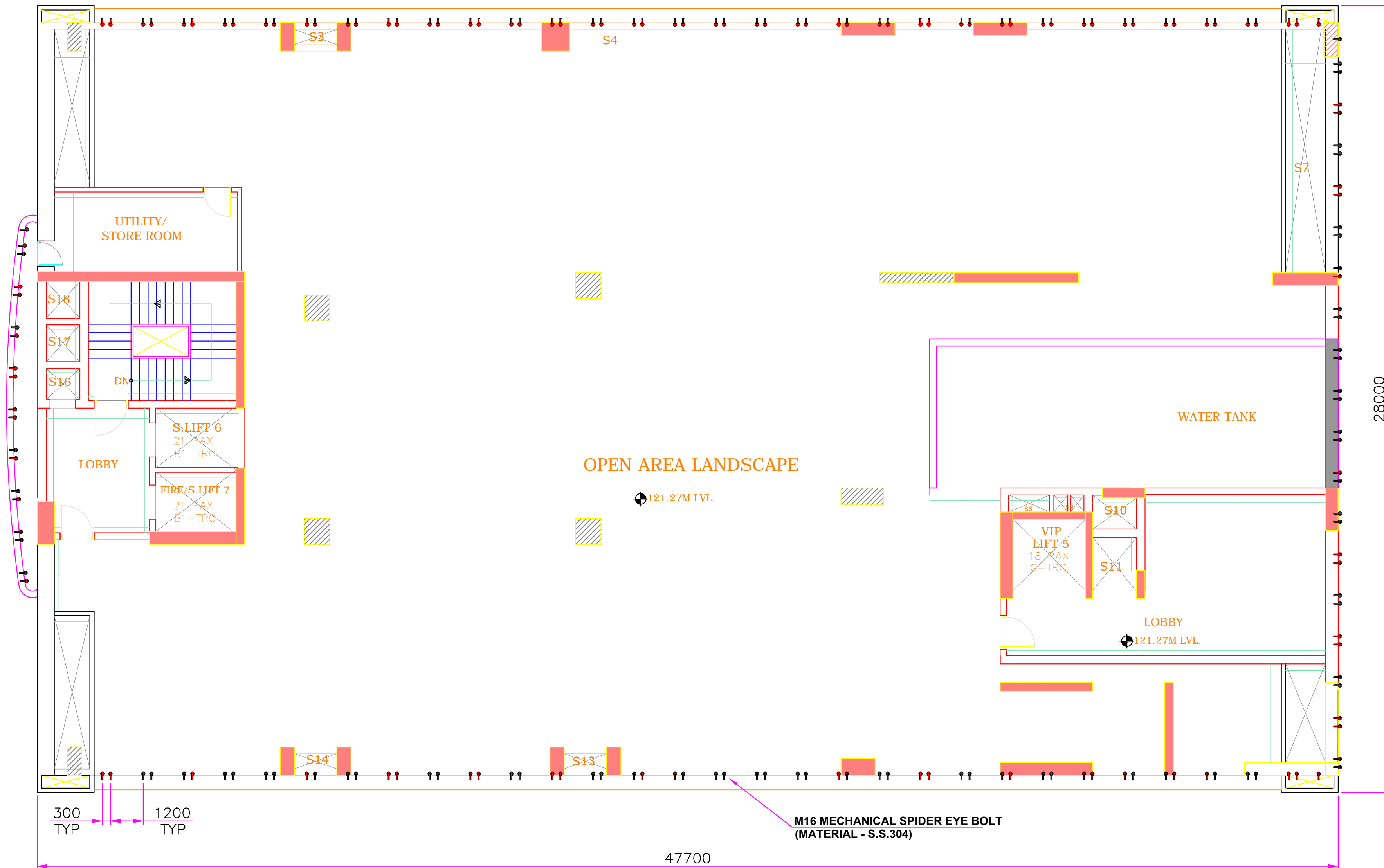
PLAN VIEW
