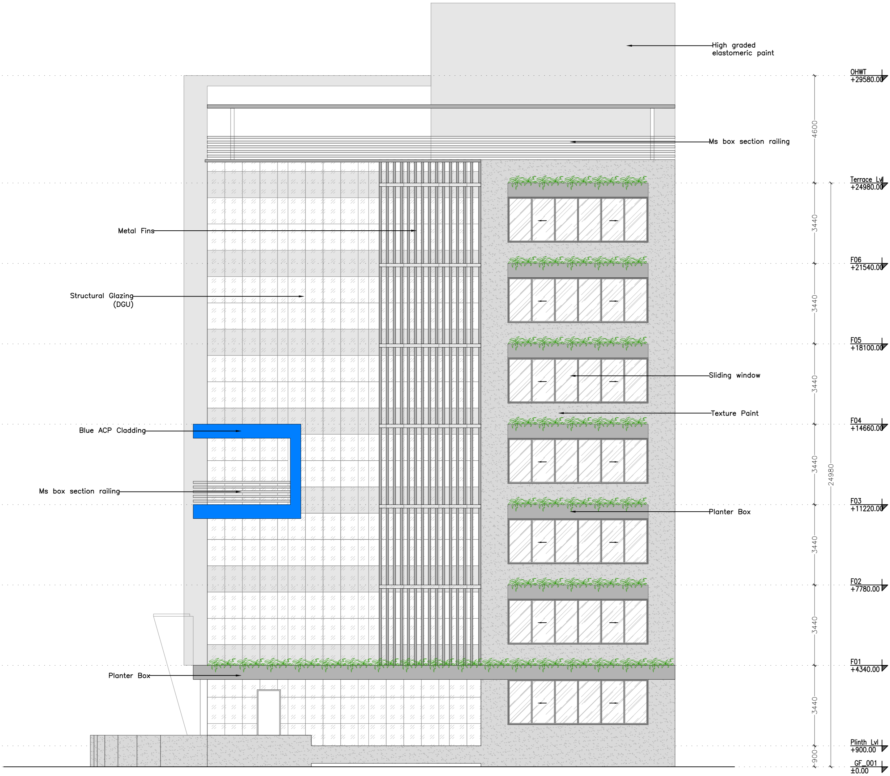
Elevation D (West Side) Scale 1:100
