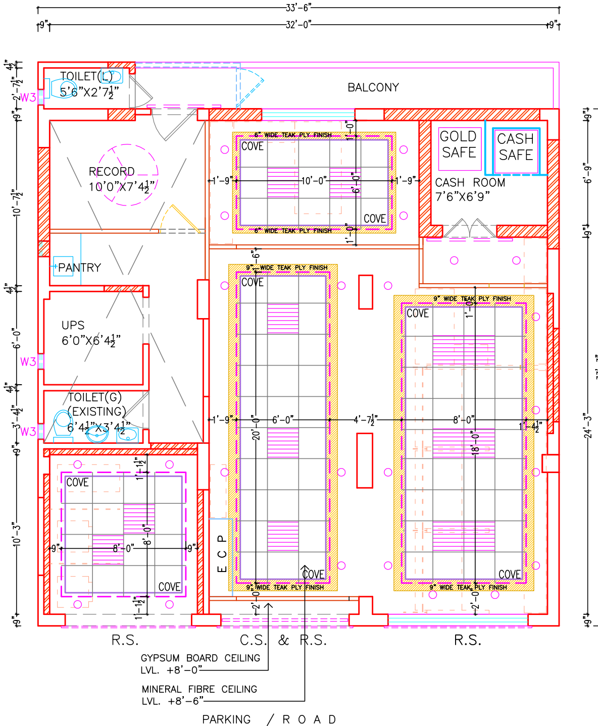
LAYOUT PLAN - G.F.
