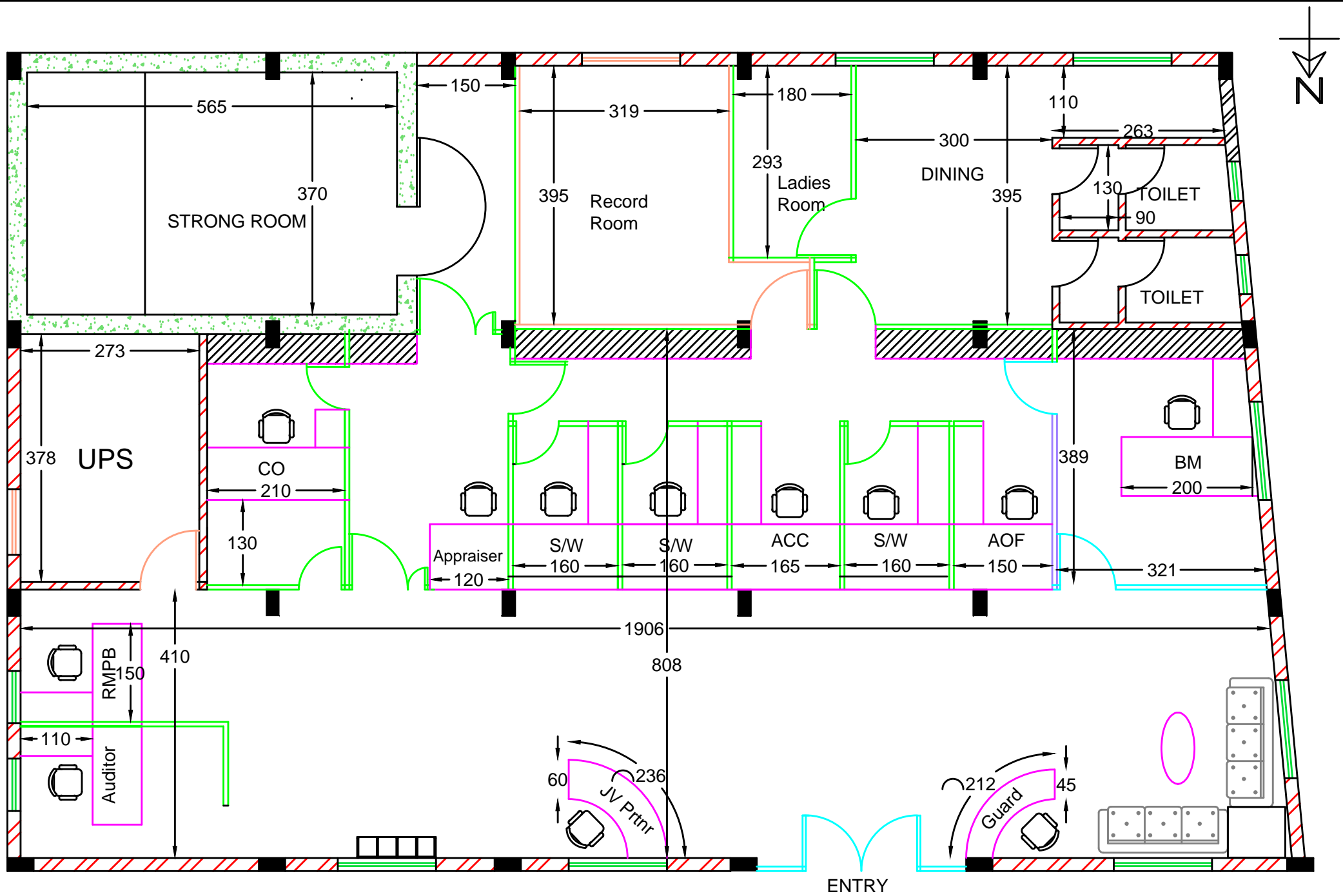
PROPOSED LAYOUT OF MUDICAL BRANCH - Option 3
