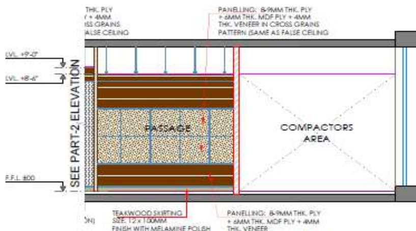
ELEVATION -1 (PART-3) (PASSAGE & COMPACTORS AREA)
