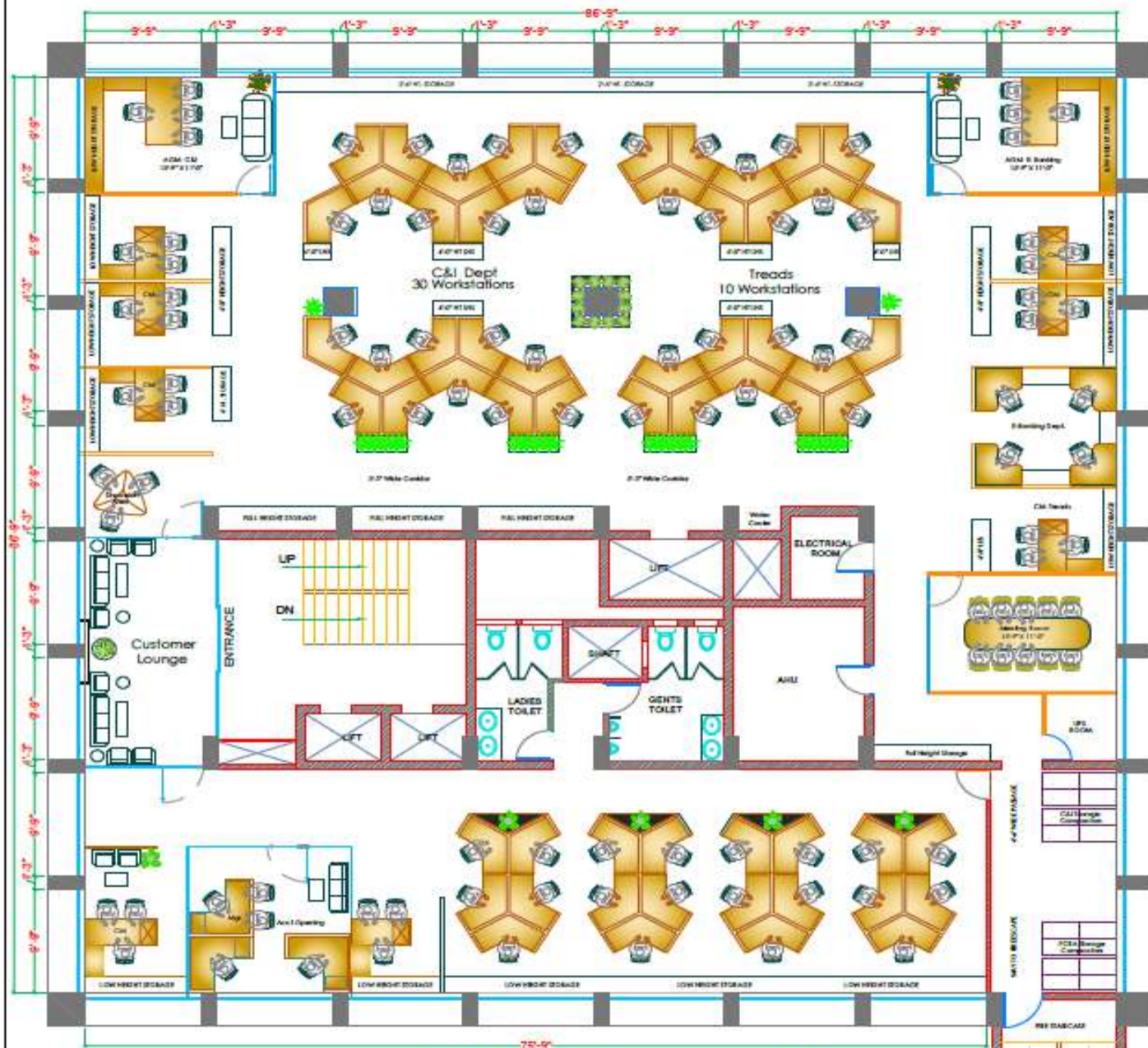
4TH Floor Proposed Layout
