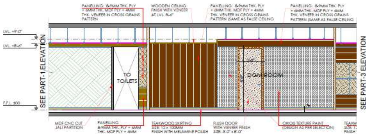
ELEVATION -1 (PART-2) (6 FT. WIDE LOBBY & DGM ROOM)
