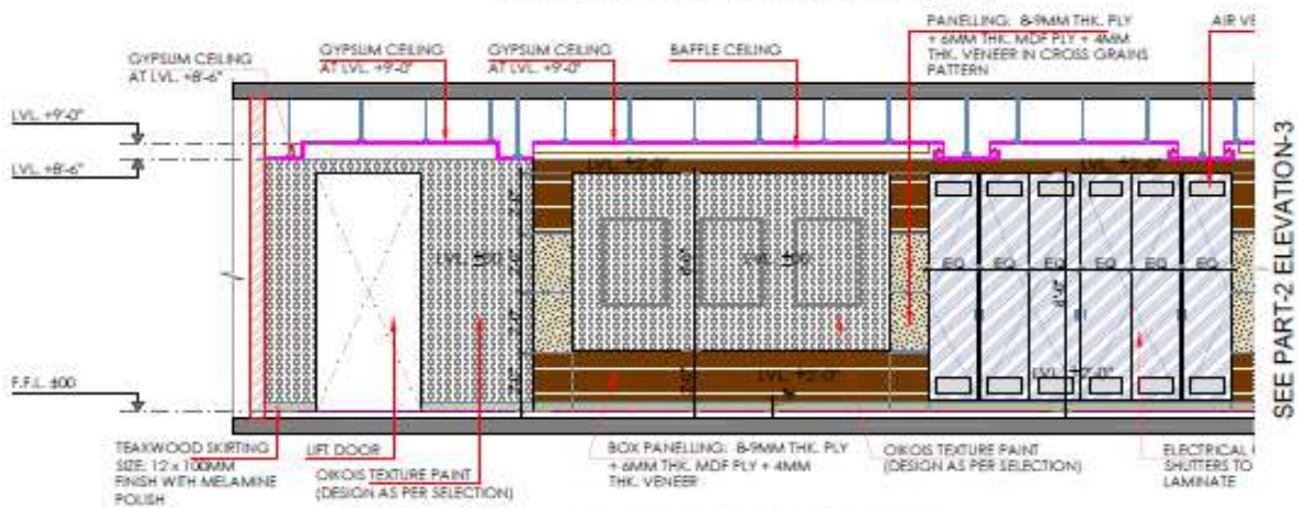
ELEVATION -3 (PART-1) (WAITING LOBBY & ELECTRICAL CABINATE)
