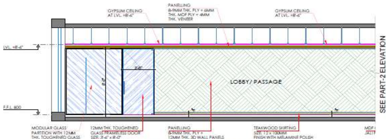
ELEVATION -1 (PART-1) (6 FT. WIDE PASSAGE LOBBY)
