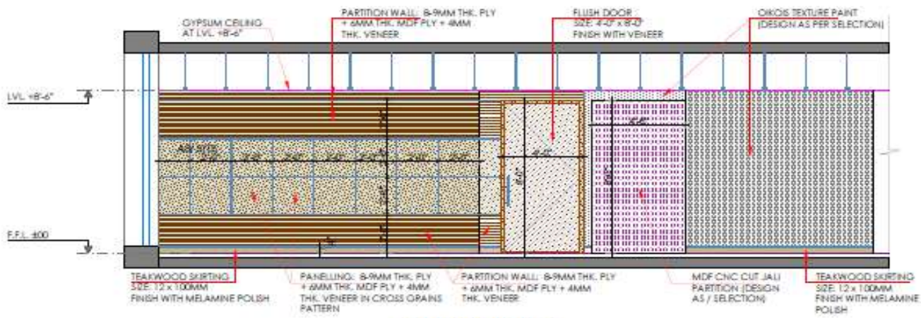
ELEVATION -2 (UPS ROOM & TOILET LOBBY)
