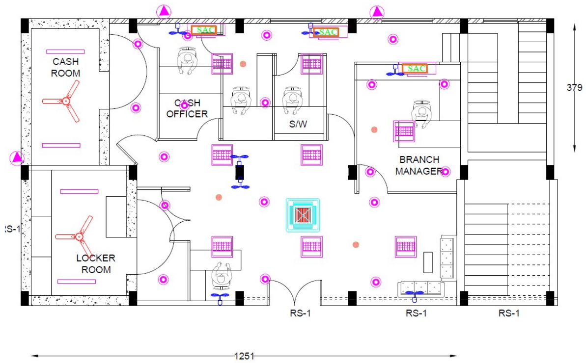
PROPOSED LAYOUT OF ERIAD BRANCH GF
