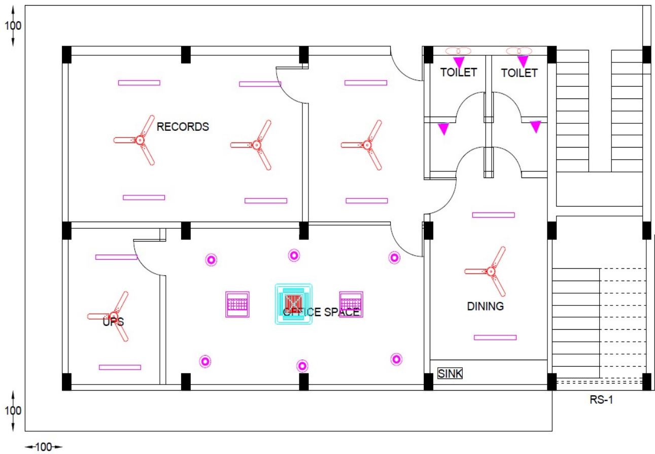
PROPOSED LAYOUT OF ERIAD BRANCH FF
