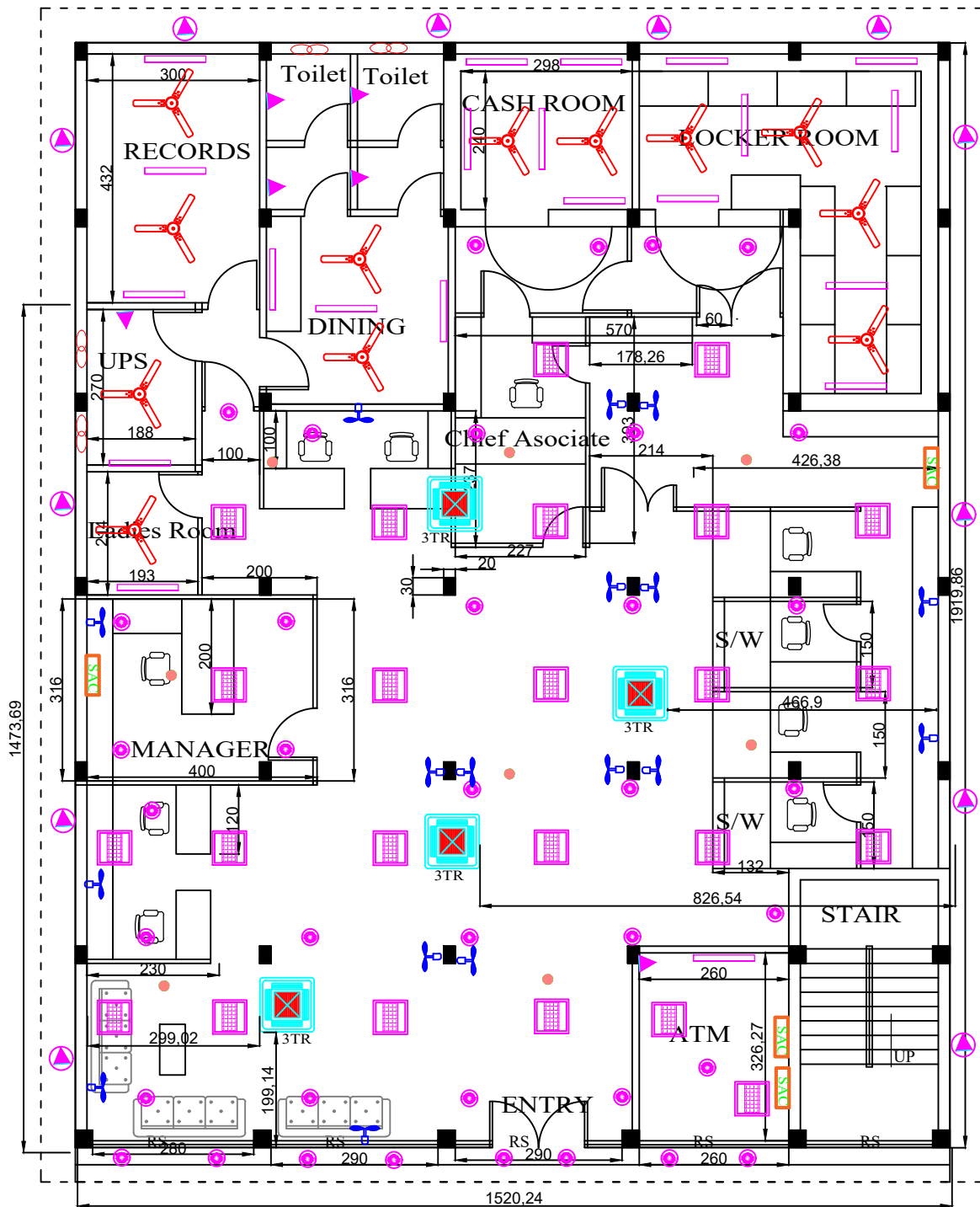
PROPOSED LAYOUT OF VALANJAMBALAM BRANCH
